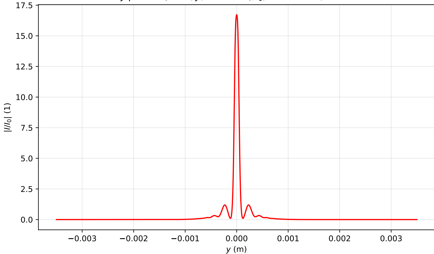
Intensity profile I(x = 0, y, z = 0.478)/I_0 , P_{in}=6.5P_{cr} , artificial time
